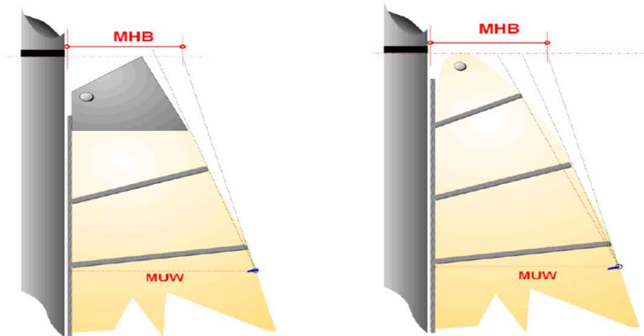
BATTENS above Upper Leech Point (Ref: IMS G.2.2)
